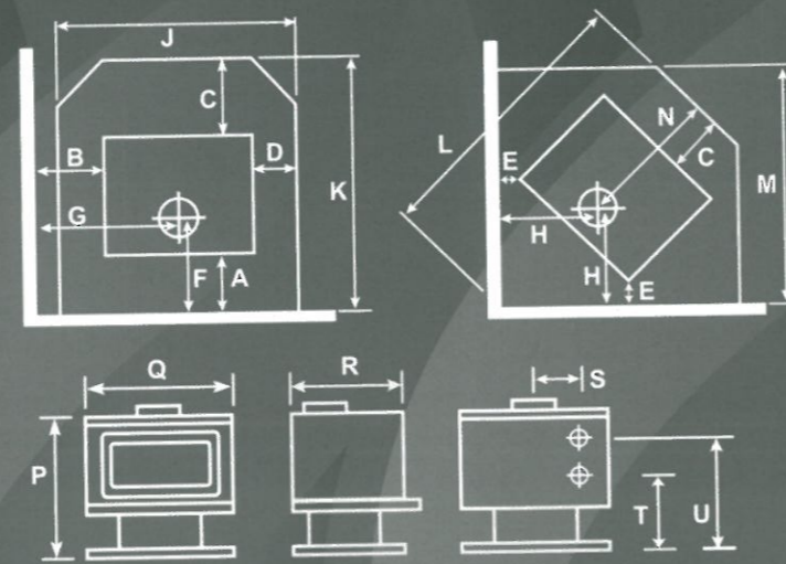
Classic CA clearance requirements with 1200mm flue shield
