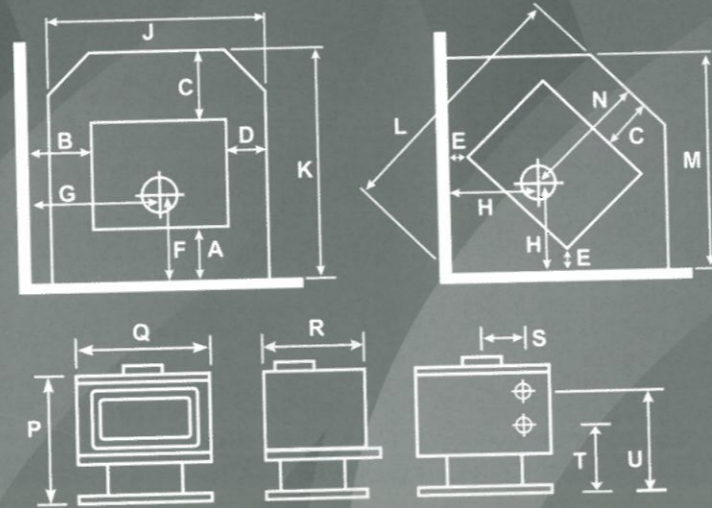
CS400 clearance requirements with 1200mm flue shield
