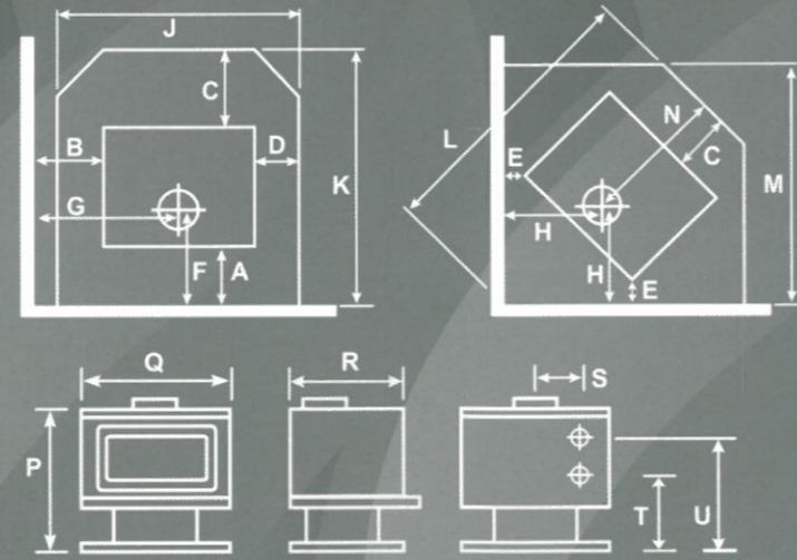
SS200 clearance requirements with 1200mm double skin flue shield
